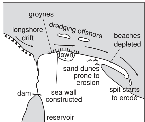
Fig. 2B Disturbed sediment cell
